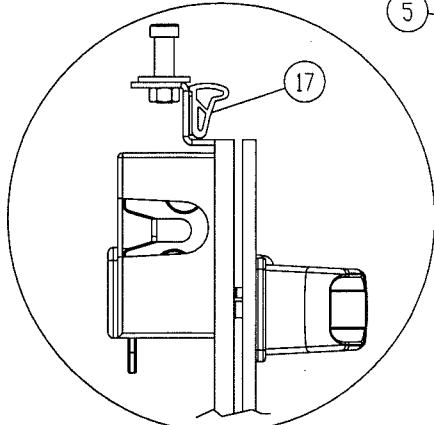
SEAL RUBBER DETAIL 2X SCALE
