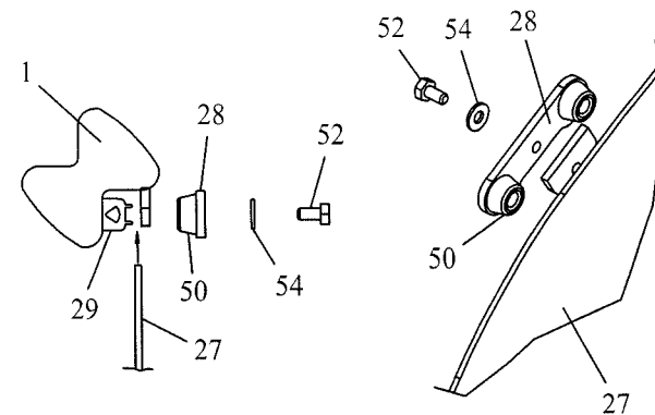
WINDOW CLAMP INSTALL 4X SCALE
