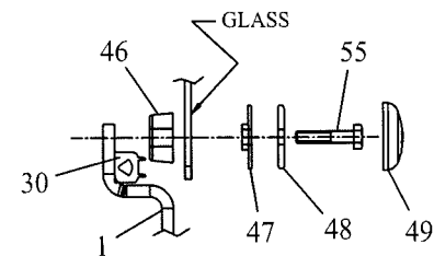
TYPICAL THROUGH GLASS BOLTING PATTERN. 4X SCALE
